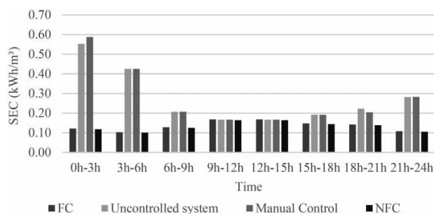
Figure 13 | Specific energy consumption.
