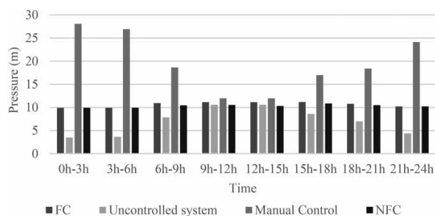
Figure 14 | Average system pressures with variable demand.
